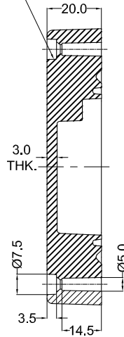
SECTION B-B
