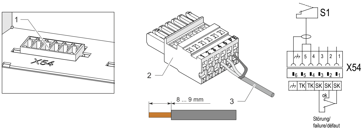
Fig. 17: Connecting a door contact switch
