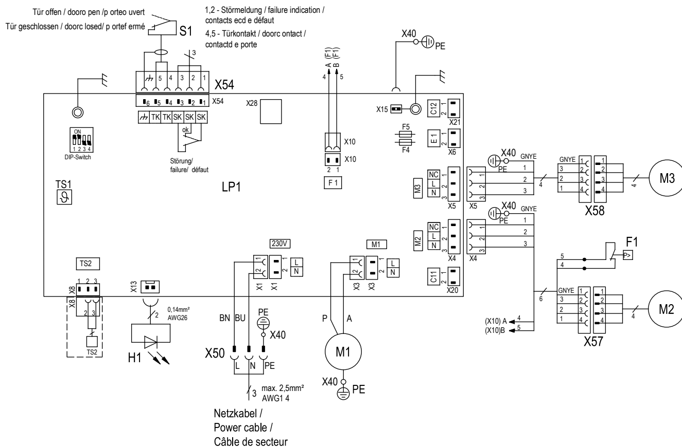
Fig. 14: Circuit diagram
