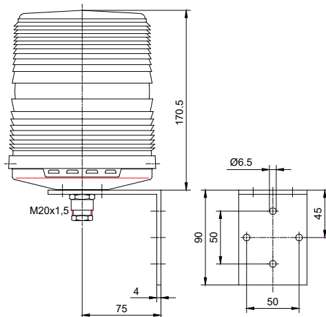
Fig. 4 Overall views
